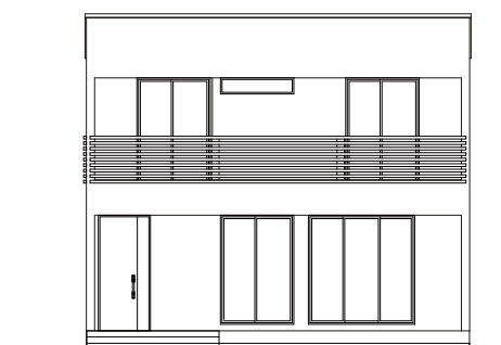
SOUTH SIDE
