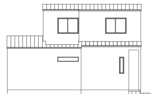
SOUTH SIDE
